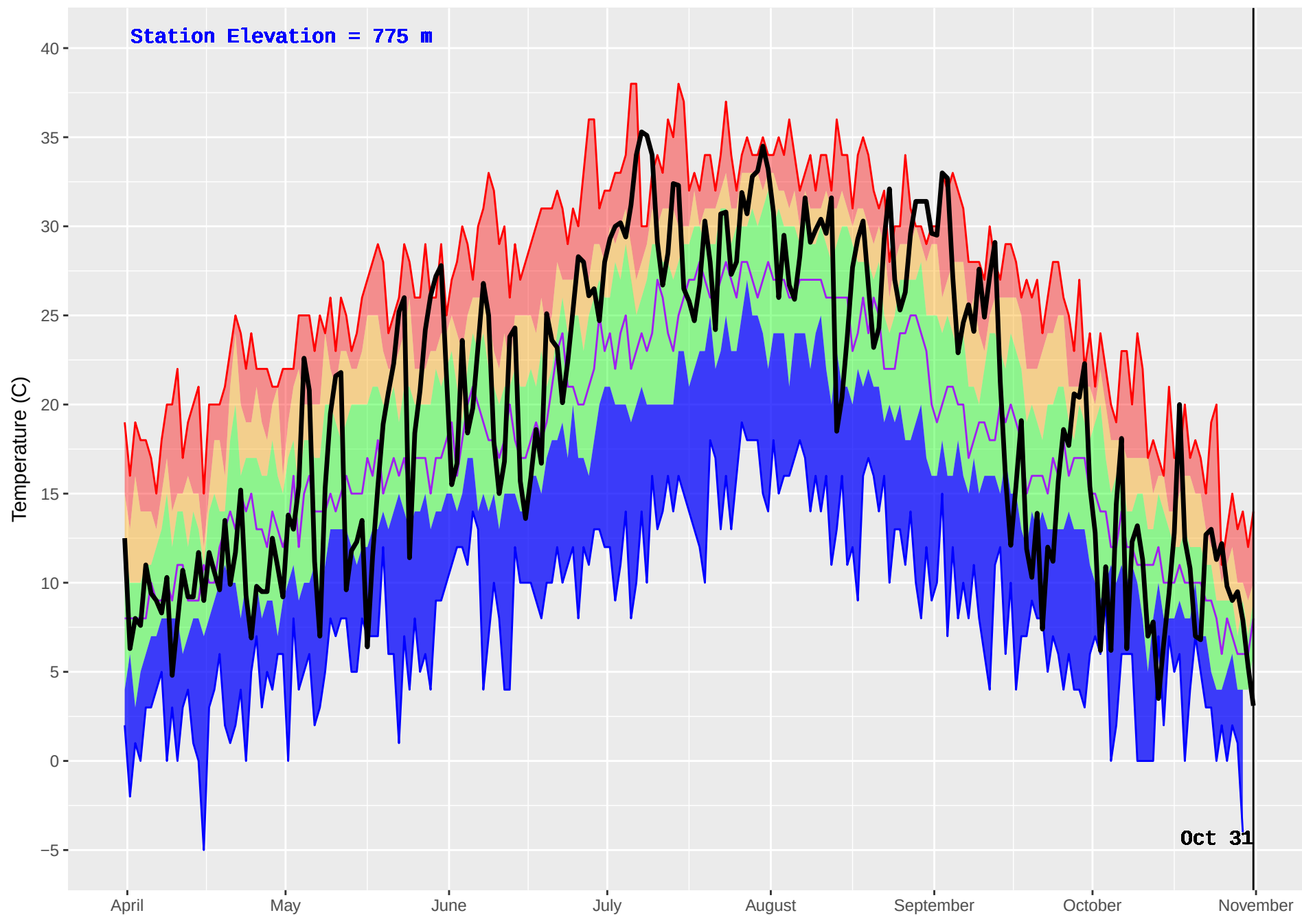
ELKO (412) : Historical (1970–2016) and Current (2017) Noon Temperature
