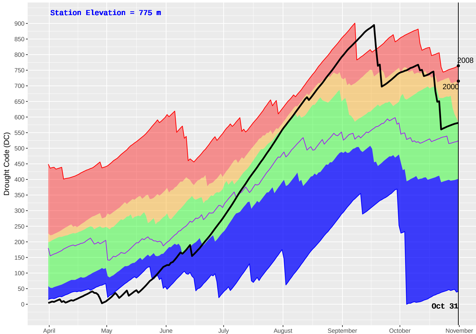
ELKO (412) : Historical (1970–2016) and Current (2017) Noon Drought Code (DC)
