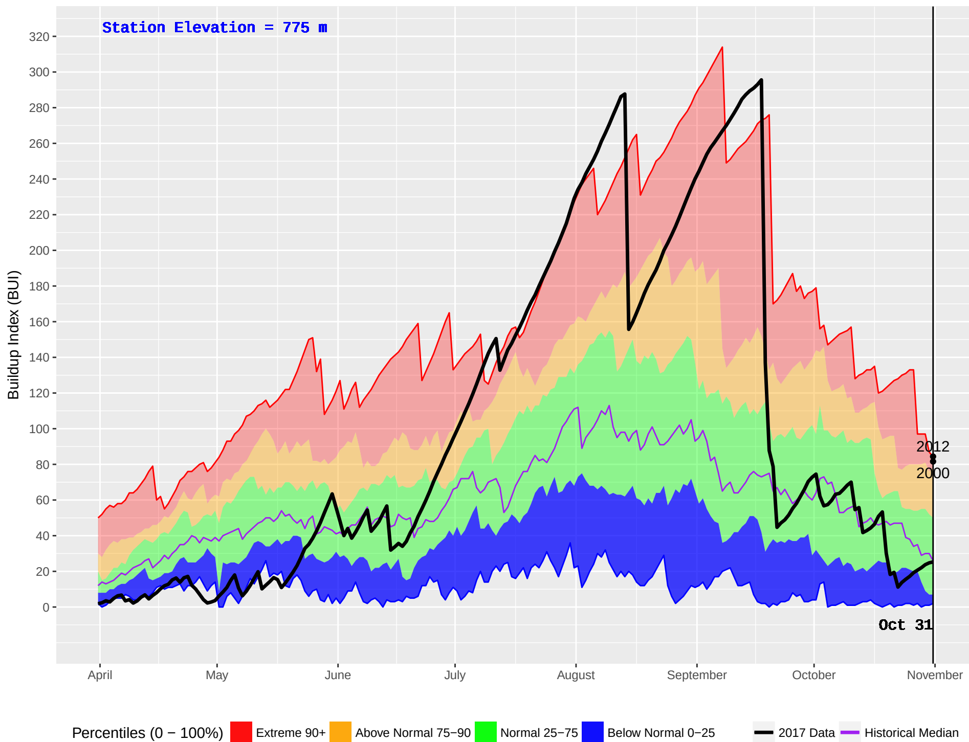
ELKO (412) : Historical (1970–2016) and Current (2017) Noon Buildup Index (BUI)
