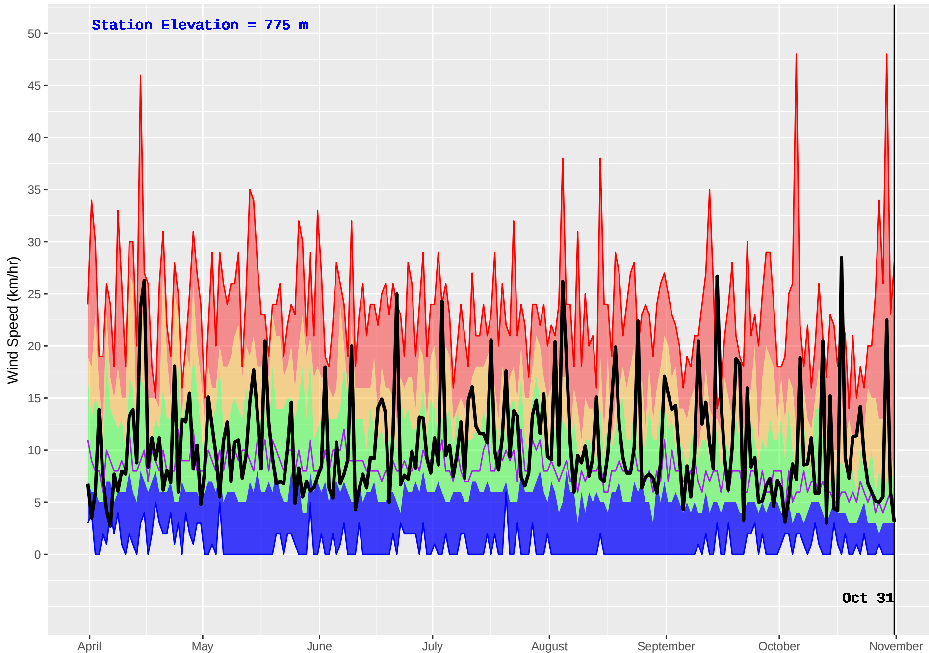
ELKO (412) : Historical (1970–2016) and Current (2017) Noon Wind Speed
