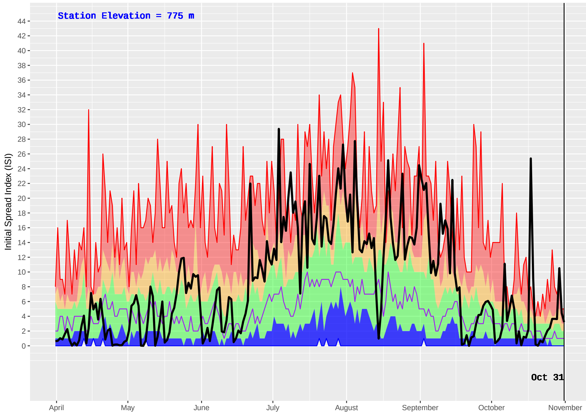
ELKO (412) : Historical (1970–2016) and Current (2017) Noon Initial Spread Index (ISI)
