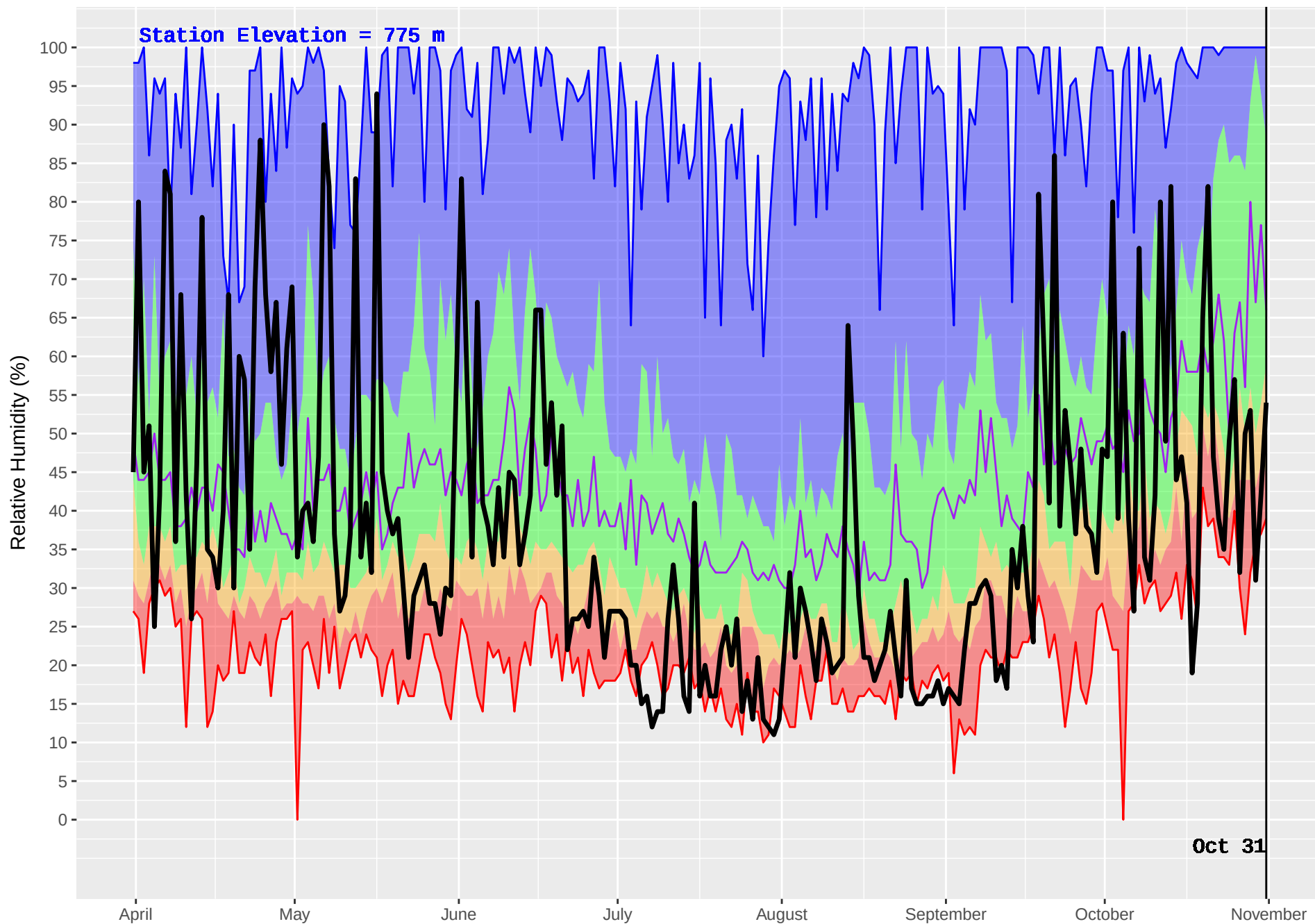
ELKO (412) : Historical (1970–2016) and Current (2017) Noon Relative Humidity
